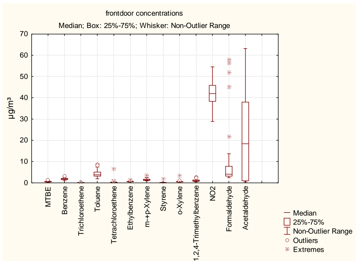
Figure 4: Boxplots of concentrations (7-days averages; expressed as µg/m 3 ) in the front door outdoor environment of 50 dwelling
