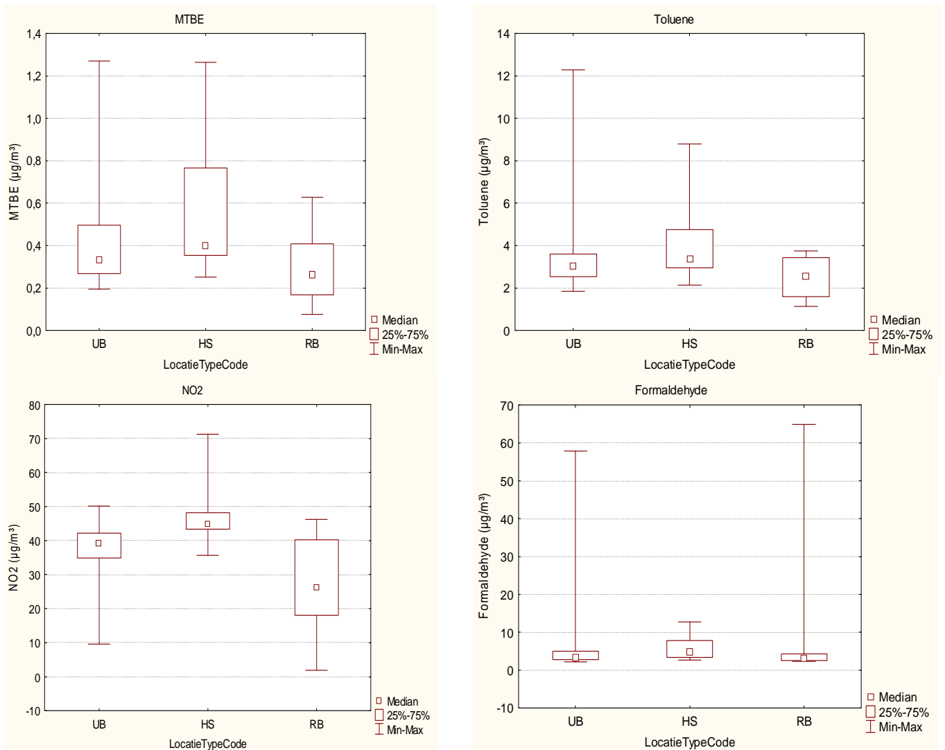
Figure 14: Comparison of outdoor concentrations (MTBE, toluene, NO 2 and formaldehyde) between urban background (UB), hot spot (HS) and rural background (RB) regions.
